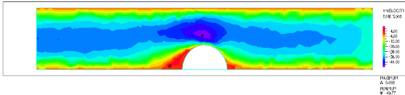
(a) Velocity in x direction at profile y = 0
